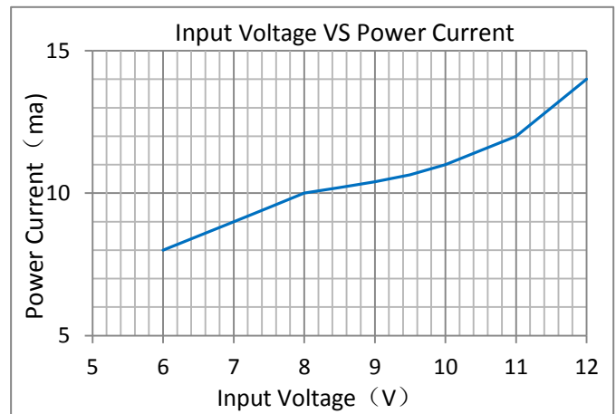
图8: Power Crrent VS. Supply Voltage
