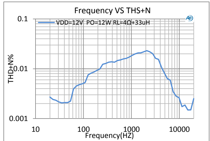
图6: Frequency VS.TH+N
